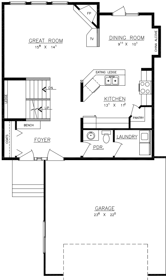
MAIN LEVEL AREA = 857 S.F.
