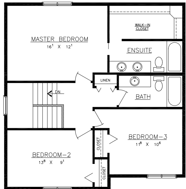
SECOND FLOOR AREA = 779 S.F.
